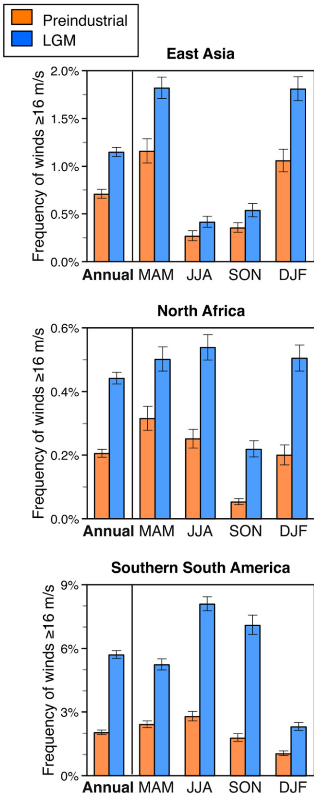
Fig. 4. Frequency of strong surface winds ( \geq 16 \text{ m s}^{-1} ) in dust source areas in preindustrial (orange) and LGM (blue) simulations using the NCAR CAM3 (Li and Battisti, 2008). Instantaneous winds were sampled twice daily in 50-year simulations of each climate state. Error bars indicate 2-sigma confidence intervals. Significant increases in strong wind gusts are observed in each dust source area during the LGM both annually and seasonally, with maximum LGM–PI differences in the winter and spring in East Asia and southern South America and in winter and summer in North Africa.
